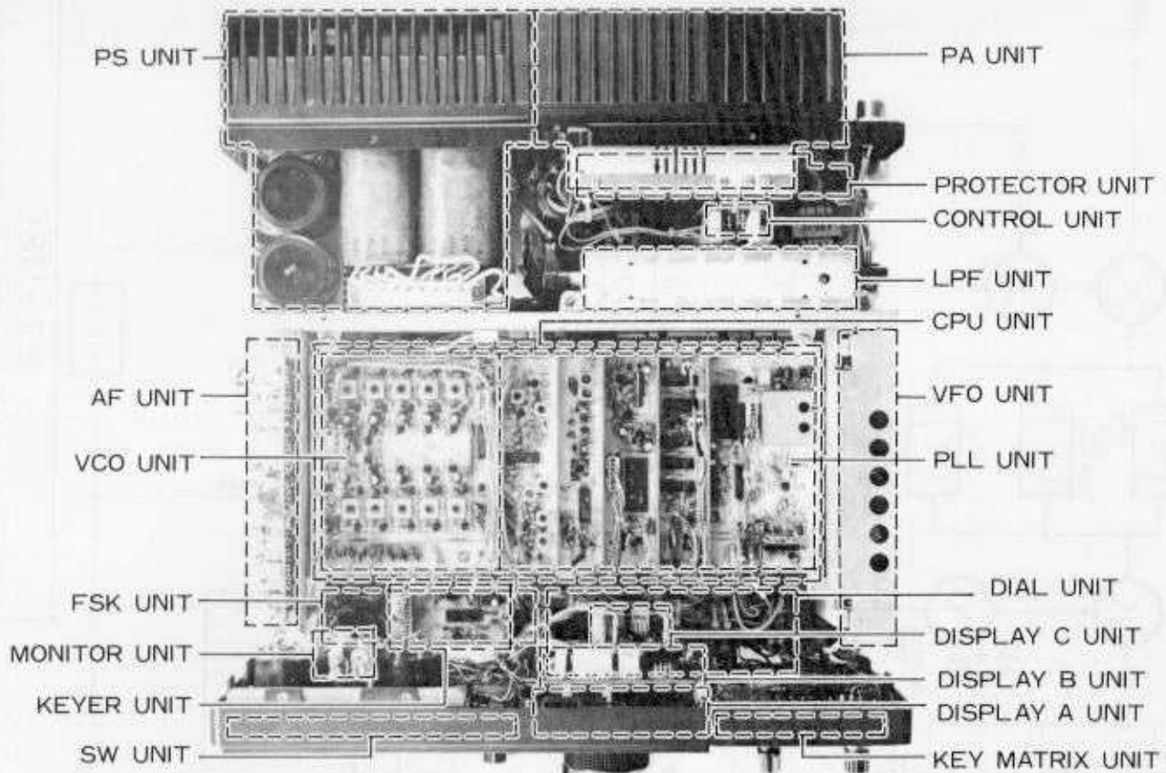
TOP VIEW
