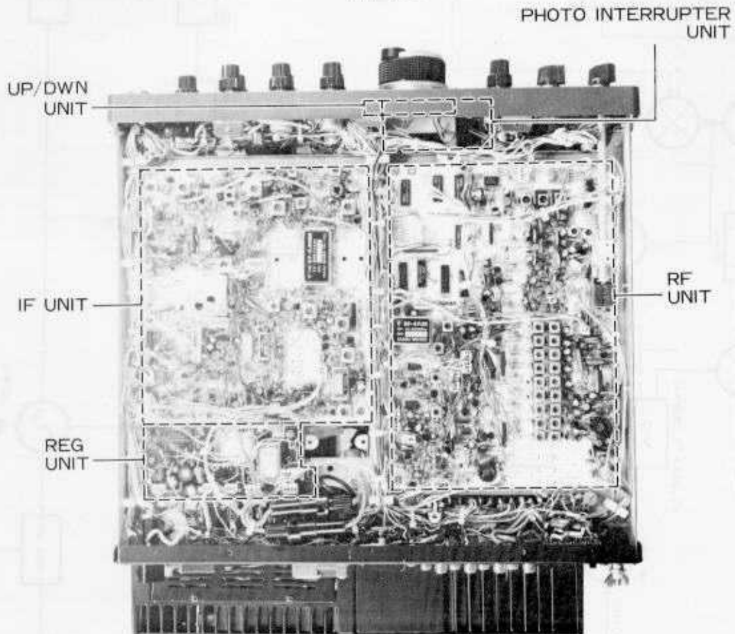
TOP VIEW
